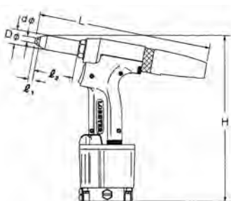
AR-2000S
